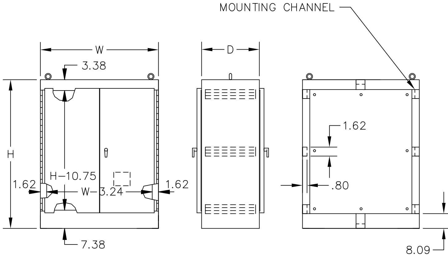
TWO DOOR DUAL ACCESS ENCLOSURES
