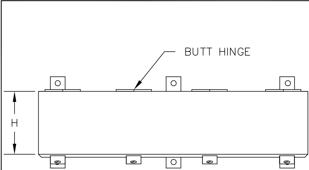
TYPE 12 HINGED COVER WIRING TROUGH
