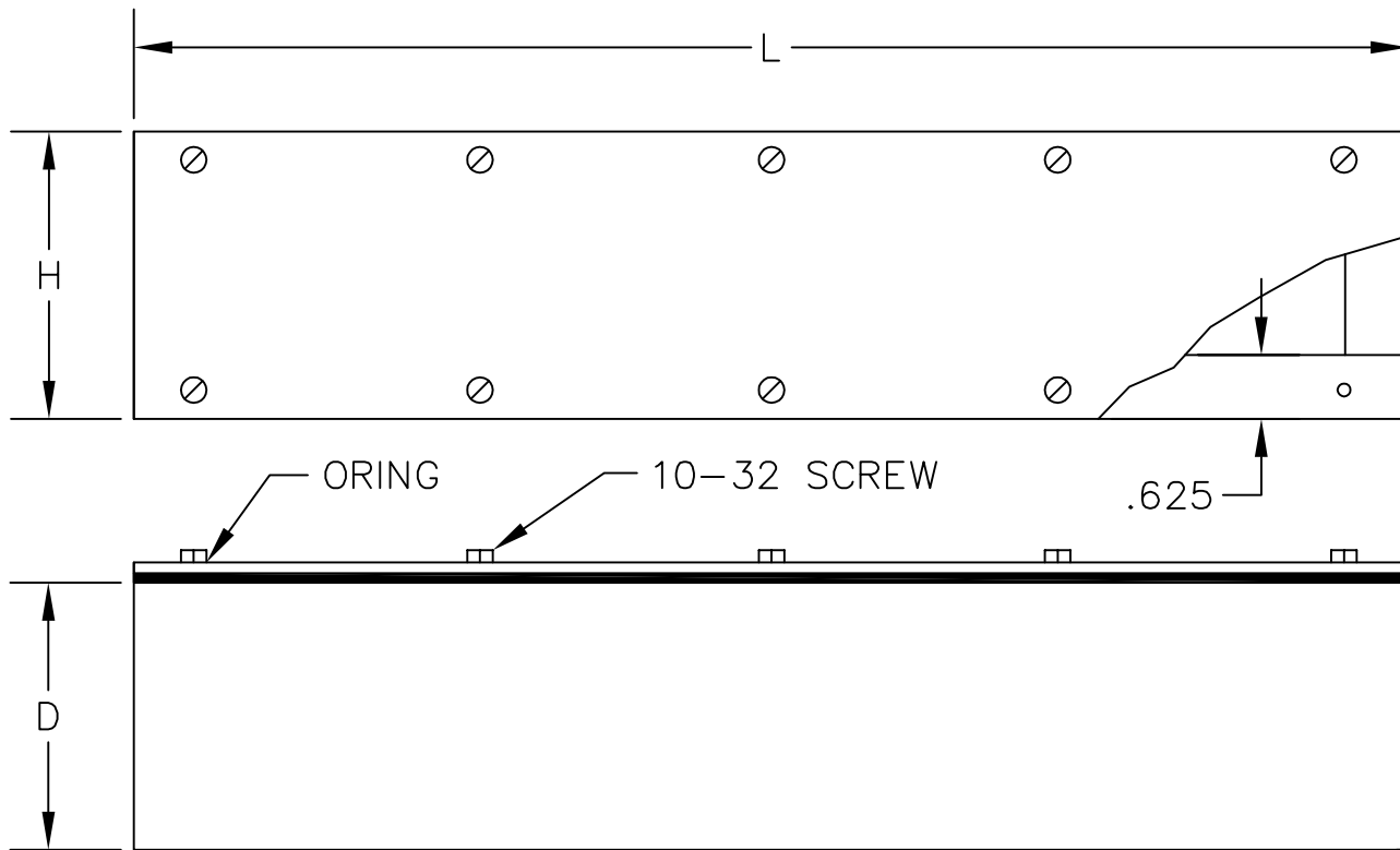
TYPE 3 AND TYPE 12 GASKETED WIRING TROUGH
