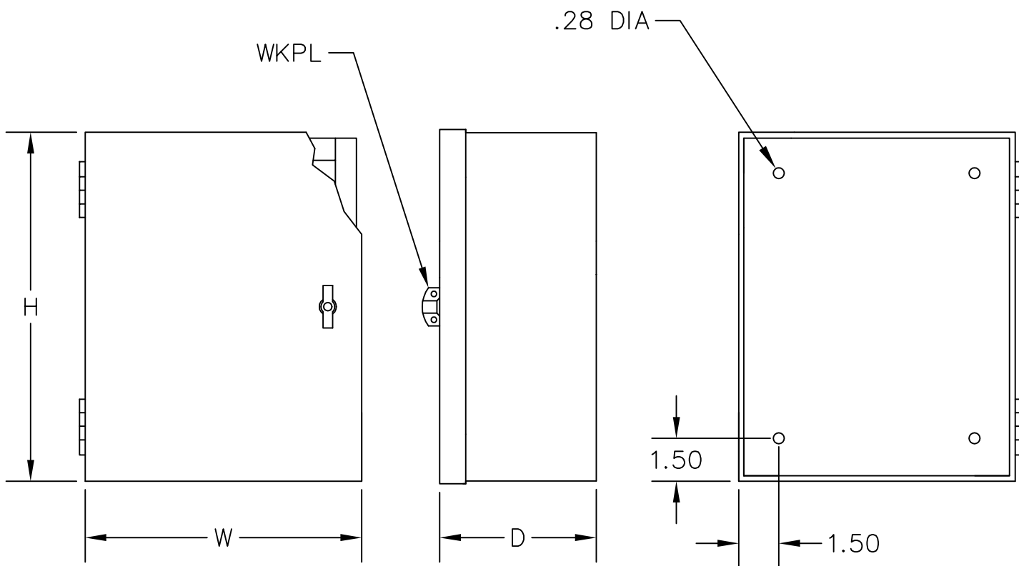
TYPE 1 CURRENT TRANSFORMER CABINETS
