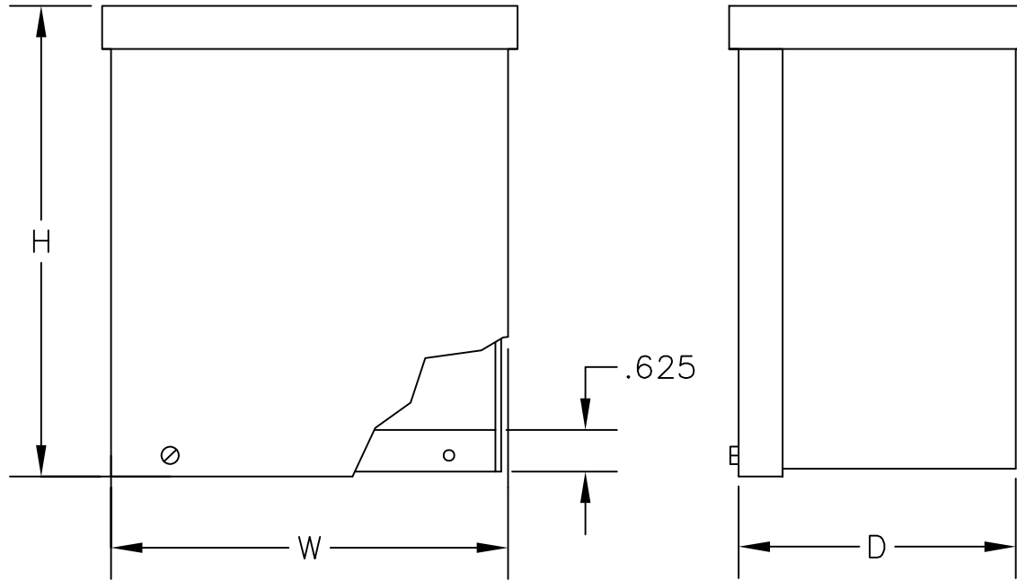
TYPE 3R RAIN-PROOF SCREW COVER
