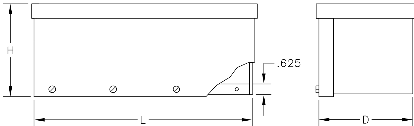
TYPE 3R RAIN-PROOF WIRING TROUGH
