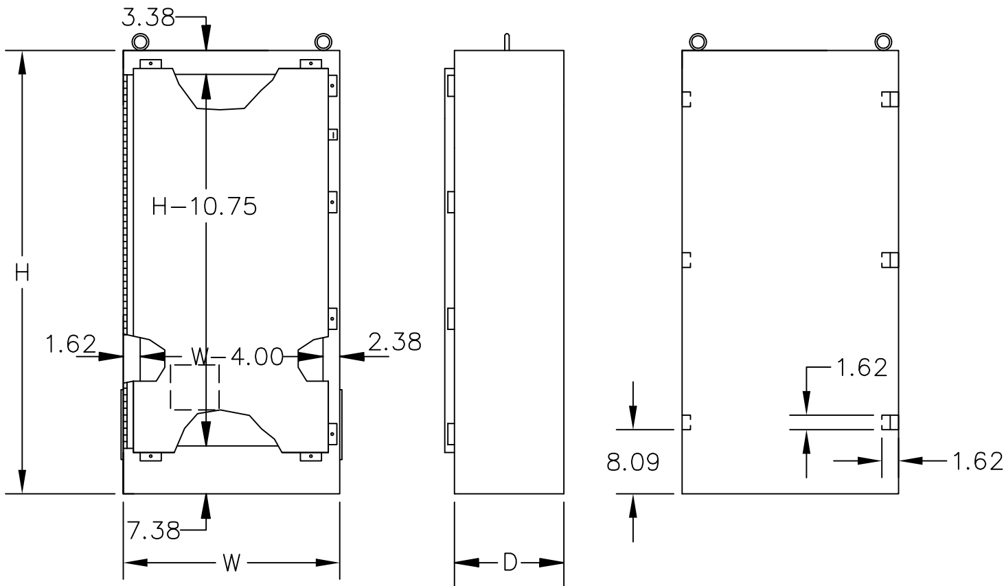
FREE STANDING TYPE 4 ENCLOSURES
