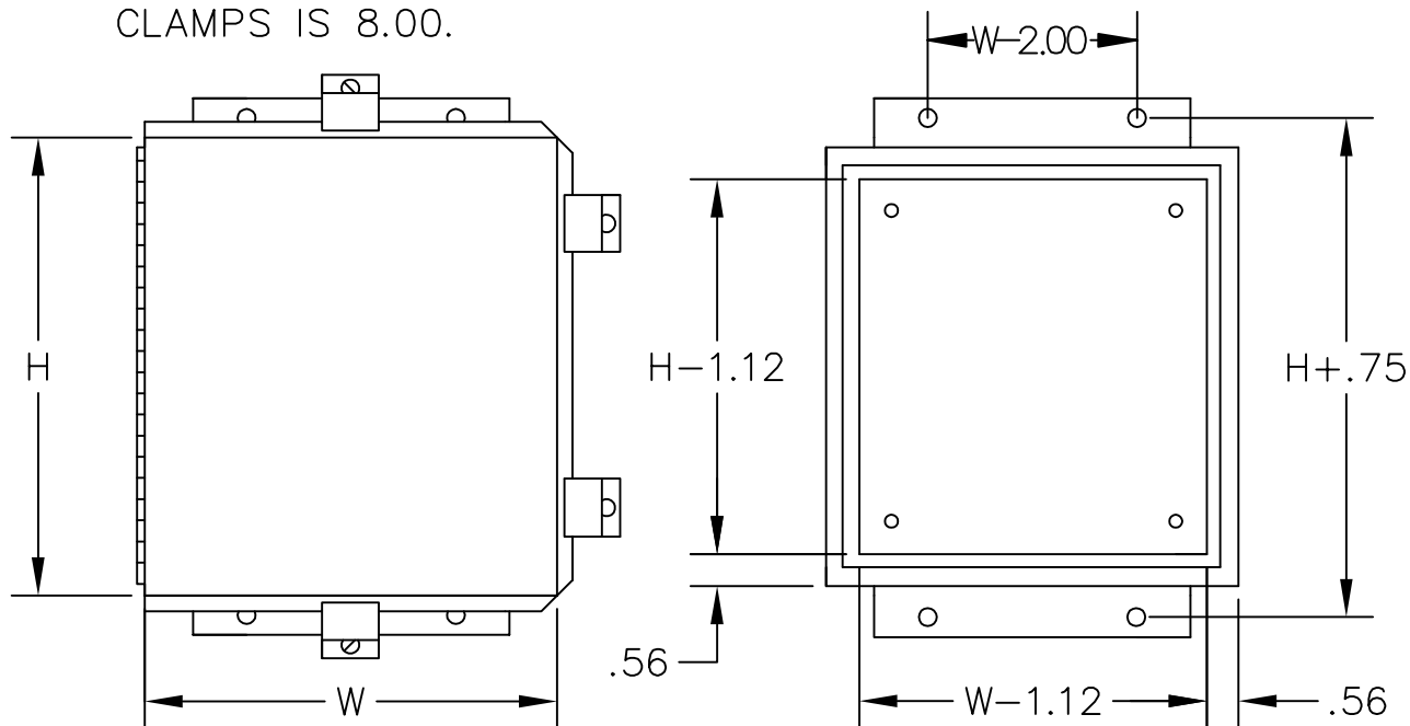
JIC HINGE COVER TYPE 4
