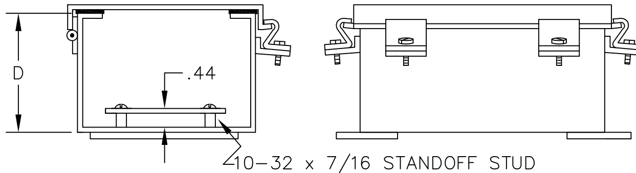
JIC HINGE COVER TYPE 4
