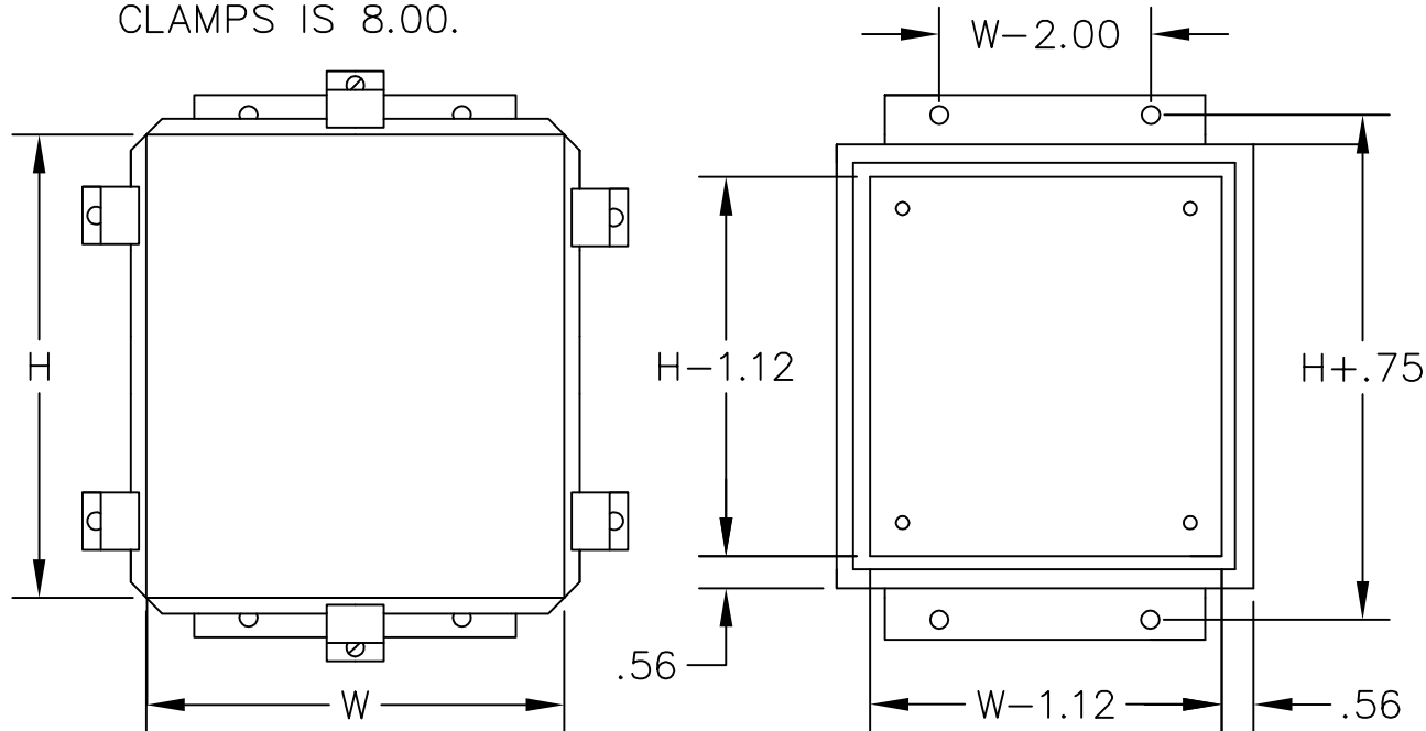
STAINLESS STEEL CLAMP COVER TYPE 4X
