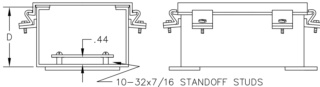
STAINLESS STEEL CLAMP COVER TYPE 4X
