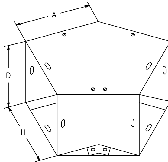
45 ELBOW
