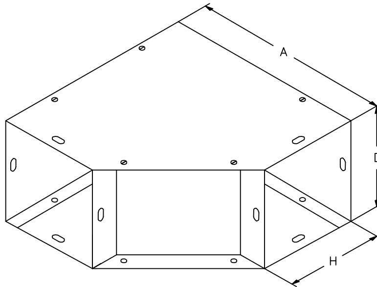
90 ELBOW
