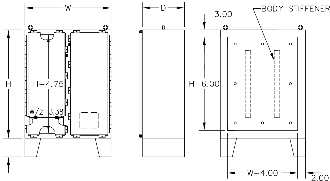
TWO DOOR TYPE 4 &amp; 4X ENCLOSURES
