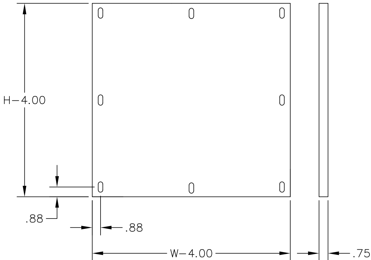
DN12 PANEL
