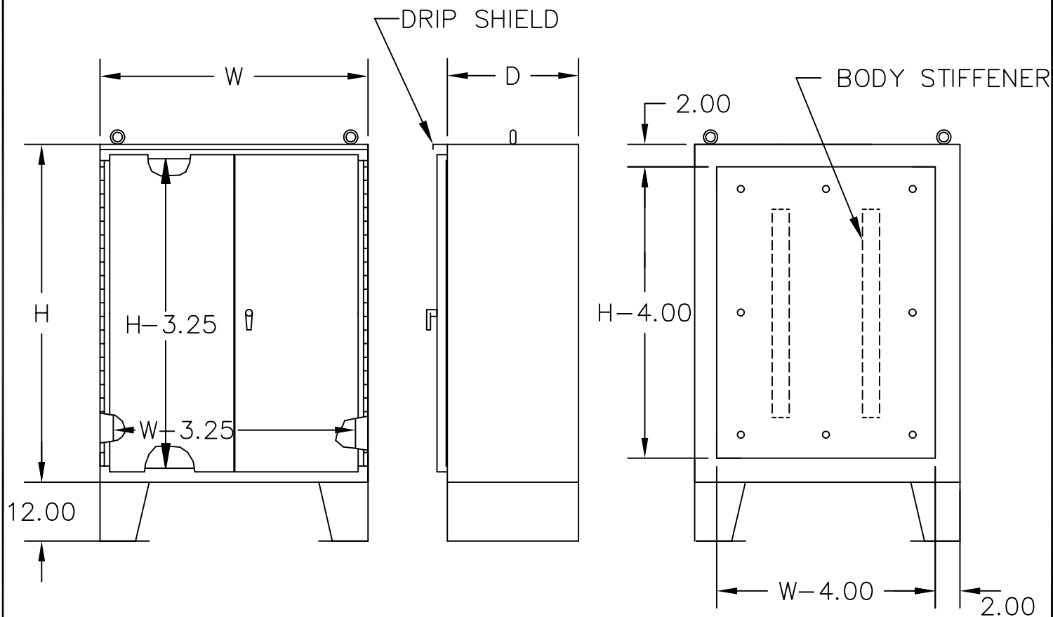
TWO DOOR TYPE 3R ENCLOSURES
