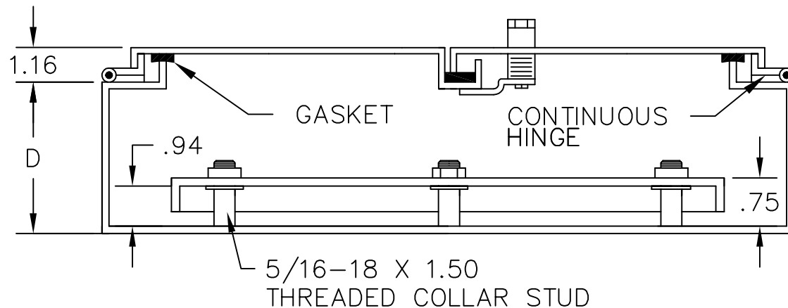
TWO DOOR TYPE 3R ENCLOSURES
