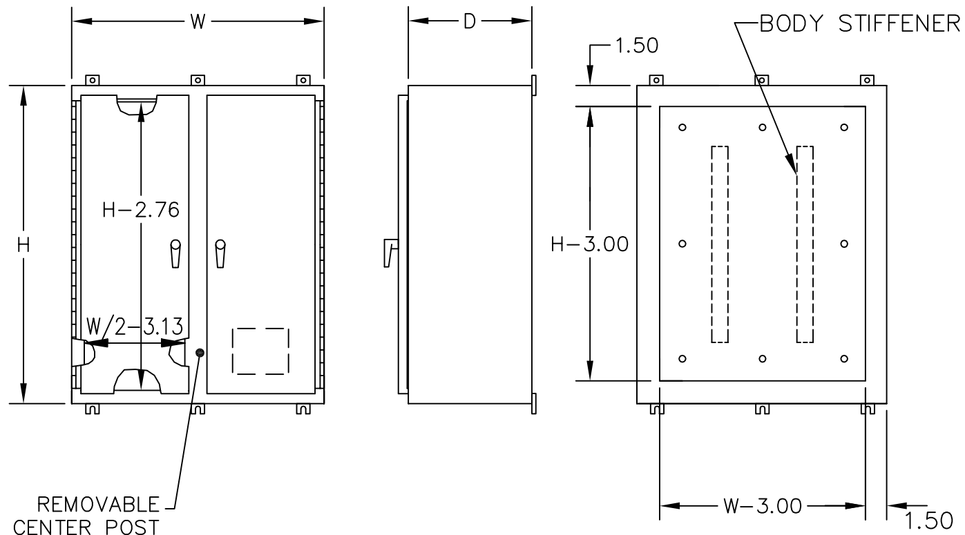
TWO DOOR TYPE 3, 3R, 12, 4 ENCLOSURES
