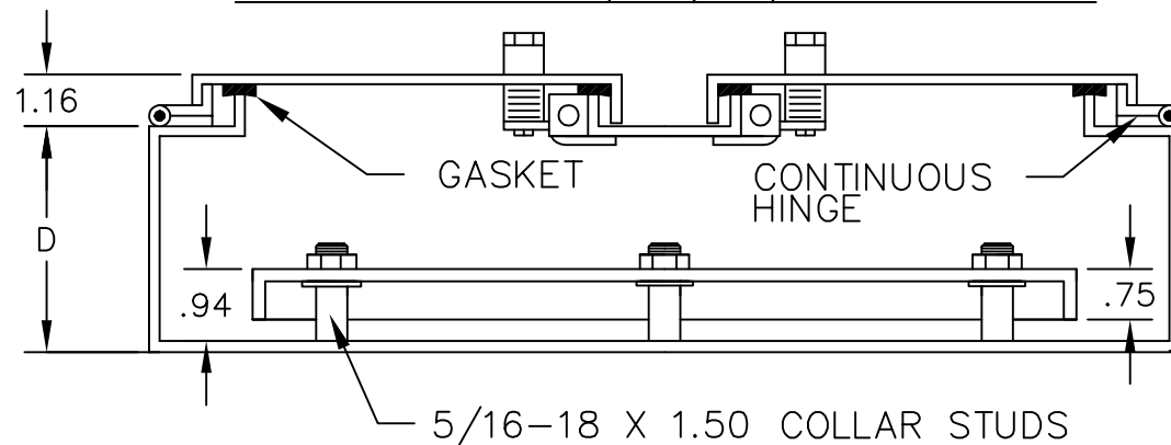
TWO DOOR TYPE 3, 3R, 12, 4 ENCLOSURES
