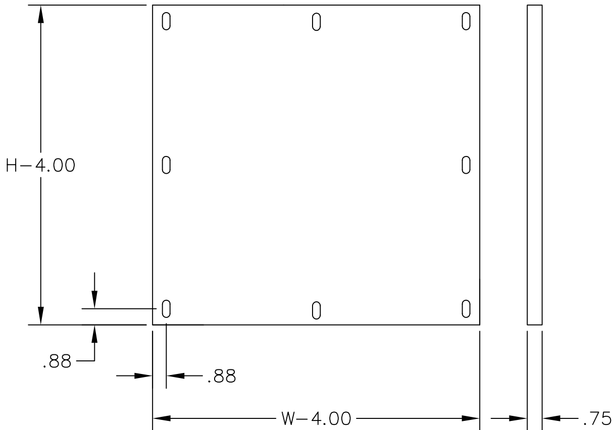
DWN12 PANEL (FOR 12 GAUGE ENCLOSURES)
