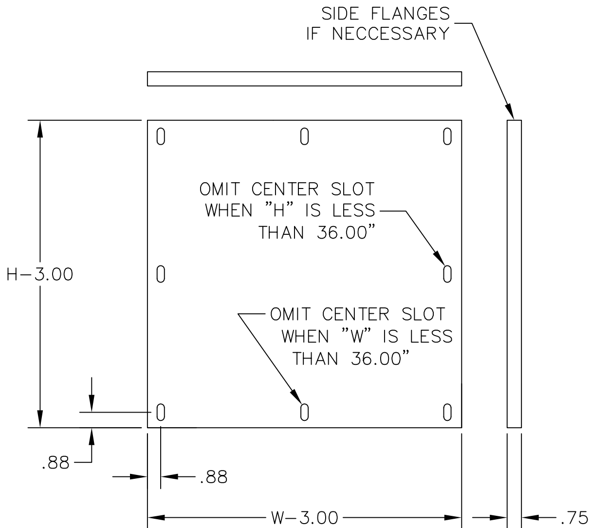
DWN12 PANEL (FOR 14 GAUGE ENCLOSURES)
