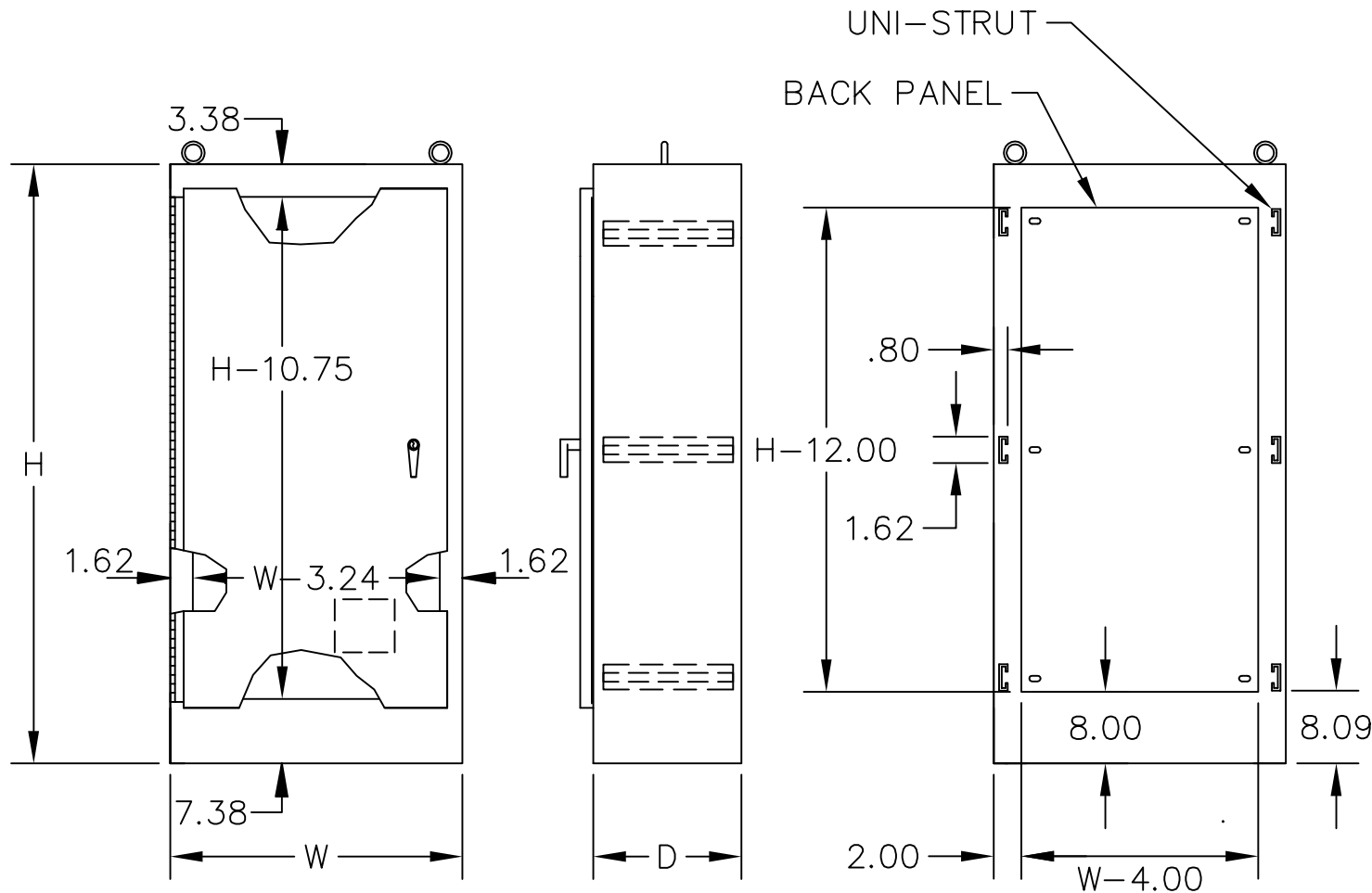
FREE STANDING TYPE 12 ENCLOSURES
