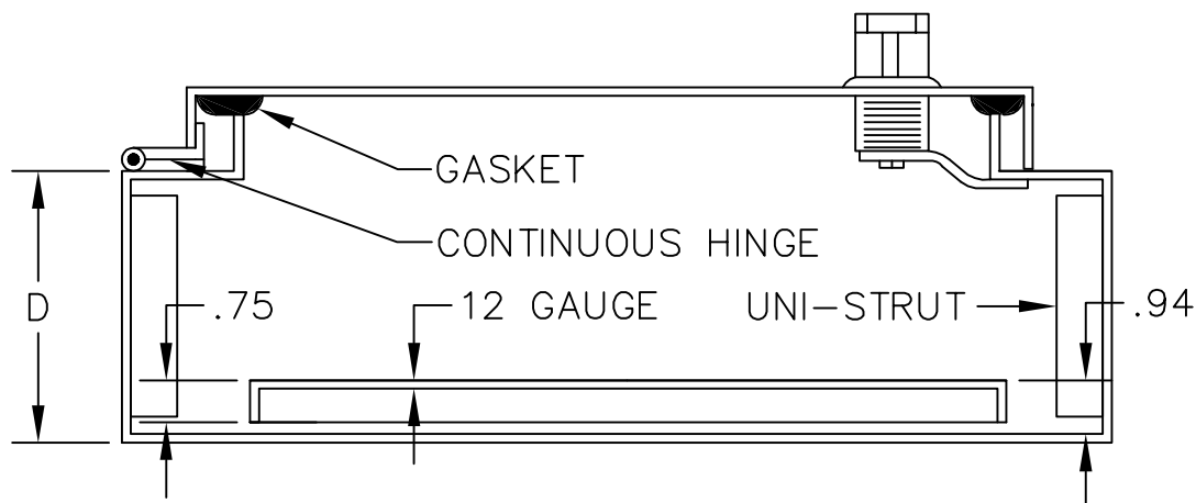
FREESTANDING SINGLE DOOR TYPE 3R, 4, 12 ENCLOSURES
