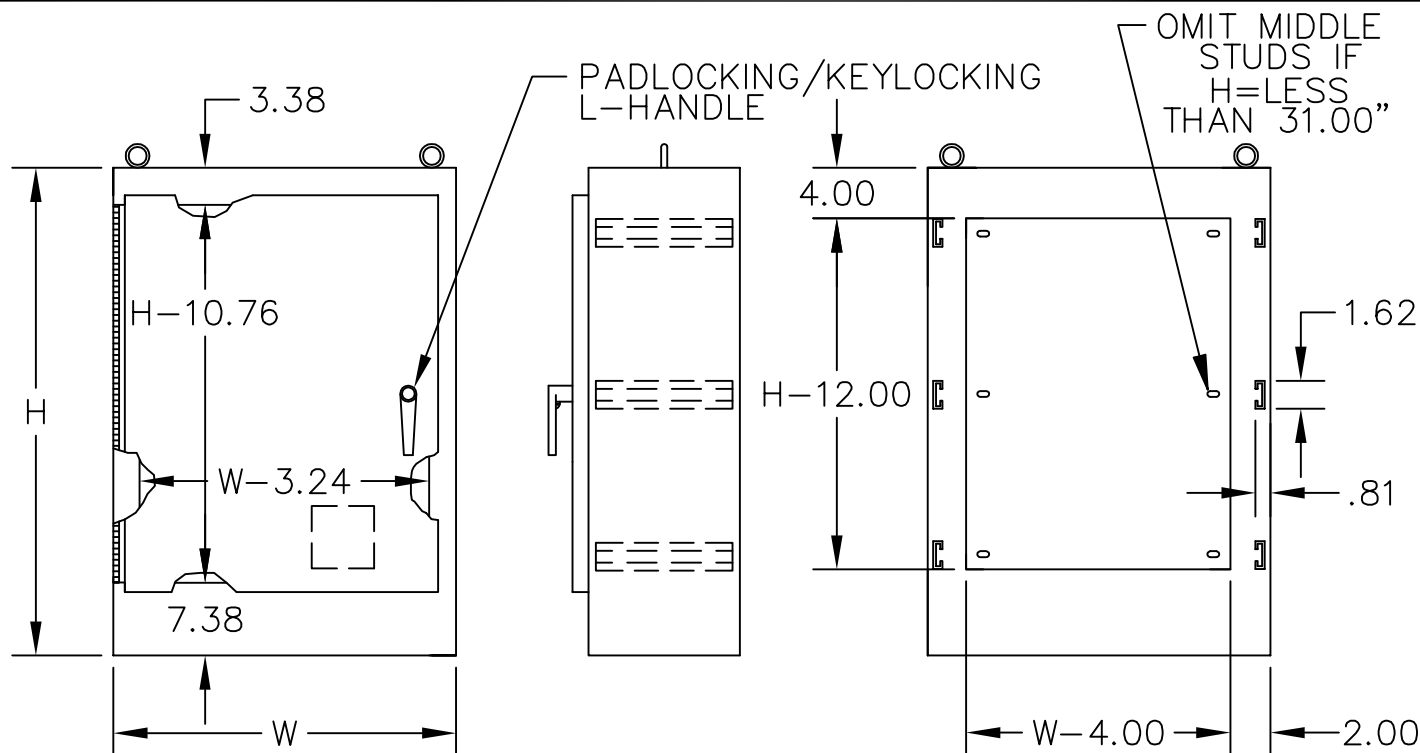
FREESTANDING SINGLE DOOR TYPE 3R, 4, 12 ENCLOSURES
