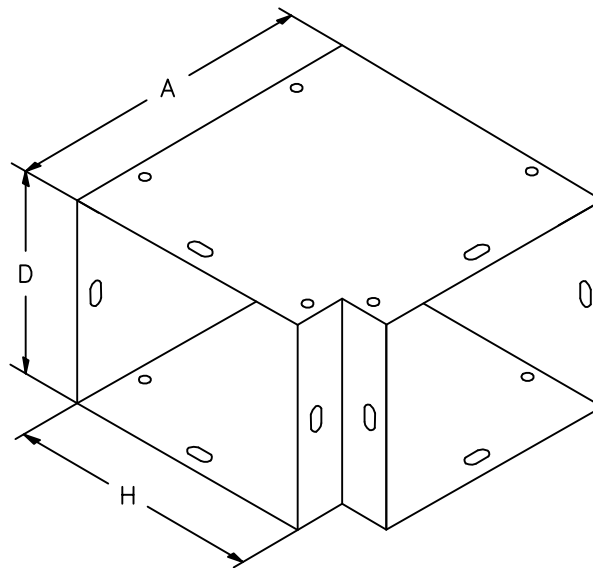
HORIZONTAL 90° ELBOW
