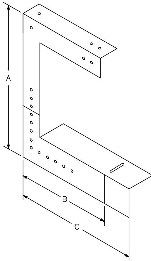
DROP HANGER
