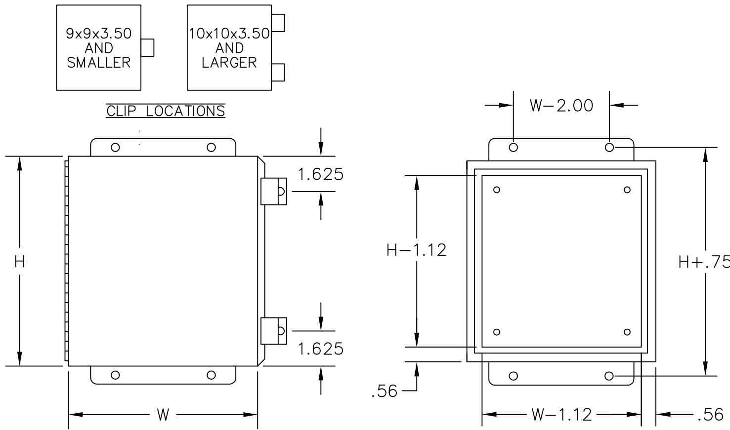
TYPE 12 & TYPE 4 JIC HINGE COVER
