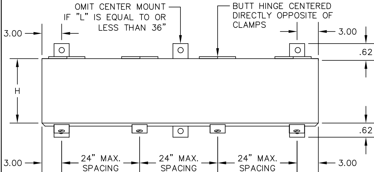
TYPE 12 HINGED COVER WIRING TROUGH
