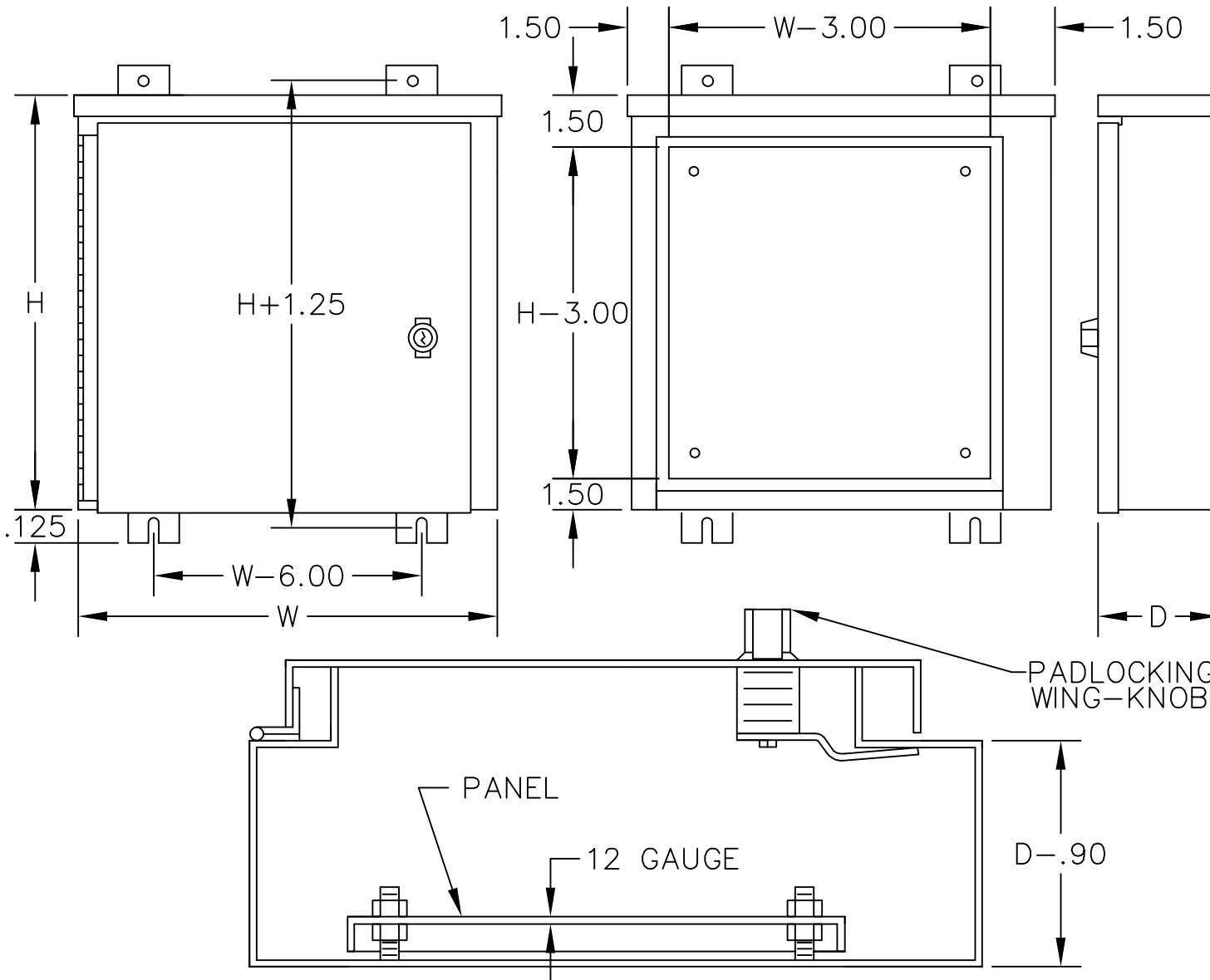
TYPE 3R HINGED ENCLOSURES
