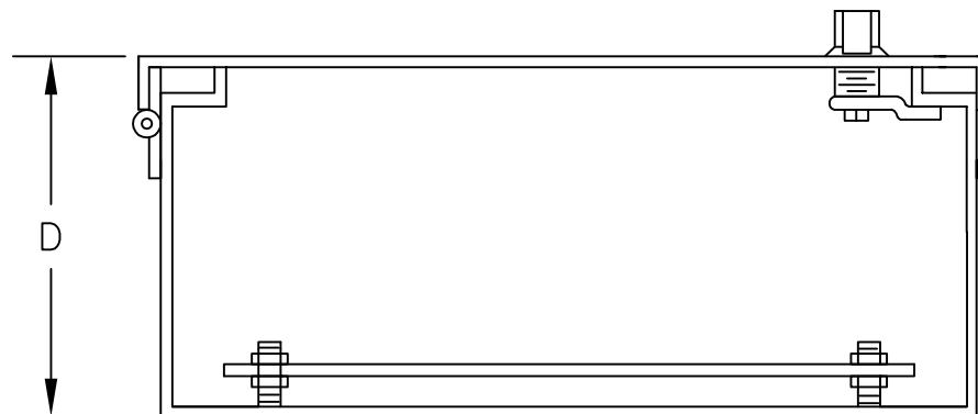
SMALL TYPE 3R RAIN-PROOF ENCLOSURES
