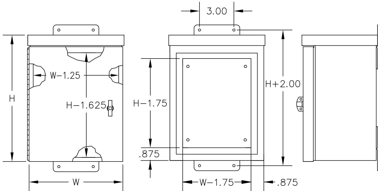
SMALL TYPE 3R RAIN-PROOF ENCLOSURES
