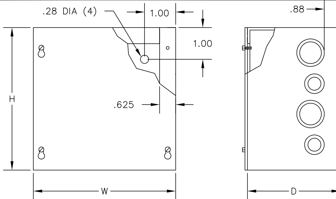
PAINTED TYPE 1 SCREW COVER BOXES WITH KNOCKOUTS
