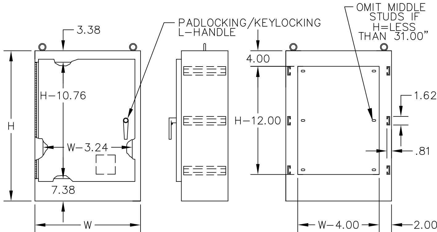
STAINLESS FREESTANDING SINGLE DOOR TYPE 3R, 4X, 12 ENCLOSURES
