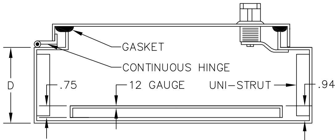
STAINLESS FREESTANDING SINGLE DOOR TYPE 3R, 4X, 12 ENCLOSURES
