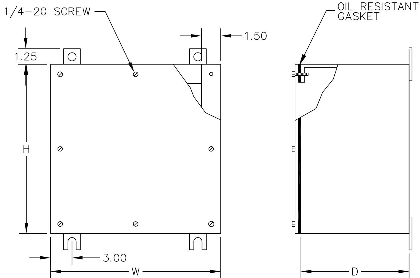
TYPE 4 GASKETED SCREW COVER
