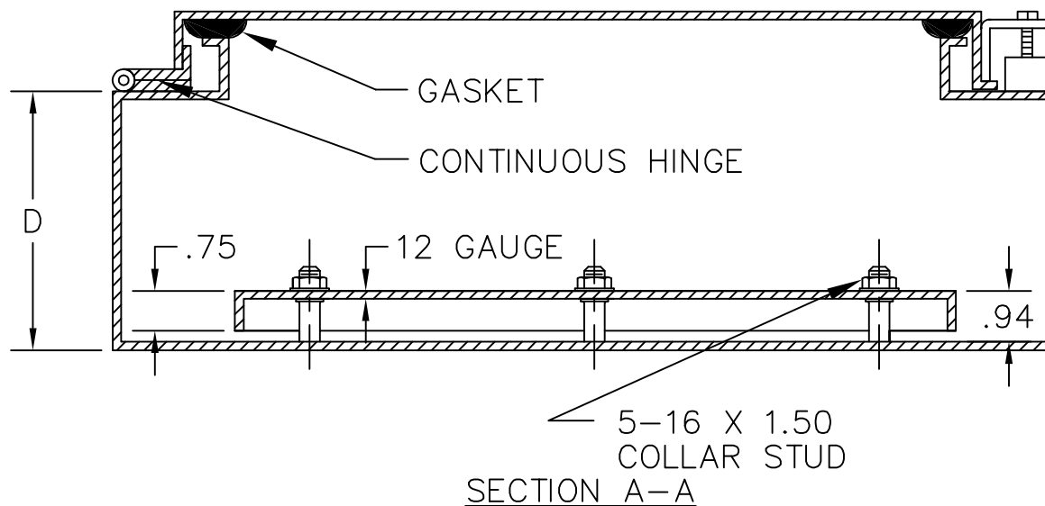
STAINLESS STEEL SINGLE DOOR TYPE 4X ENCLOSURES
