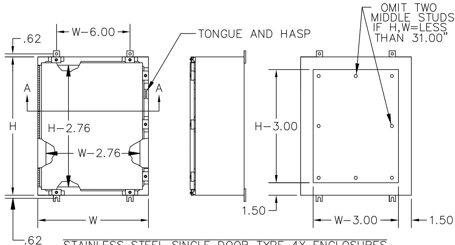
STAINLESS STEEL SINGLE DOOR TYPE 4X ENCLOSURES
