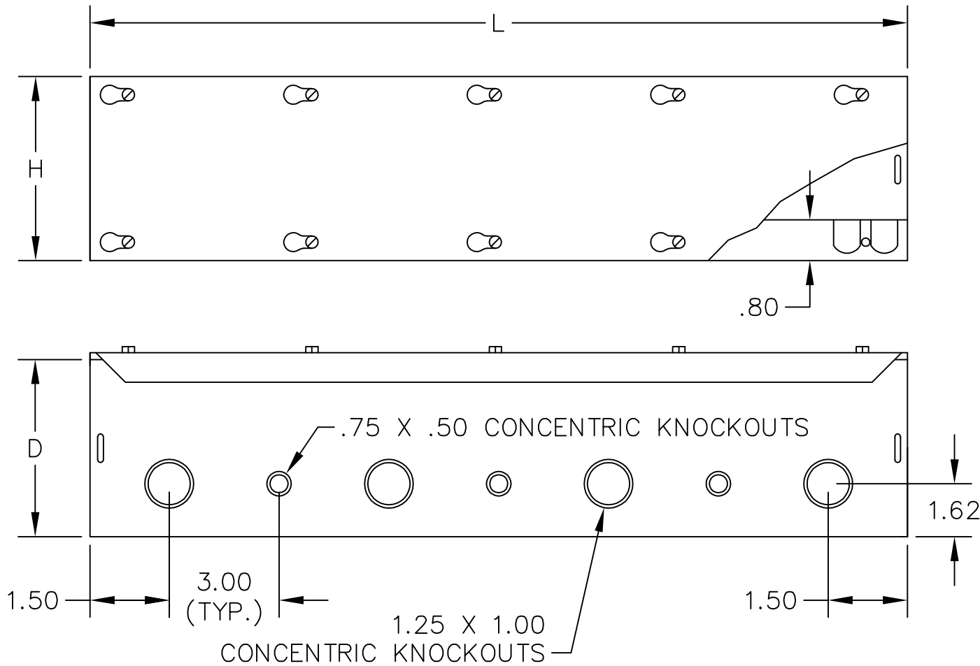
TYPE 1 SCREW COVER WIREWAY (WITH KNOCKOUTS)
