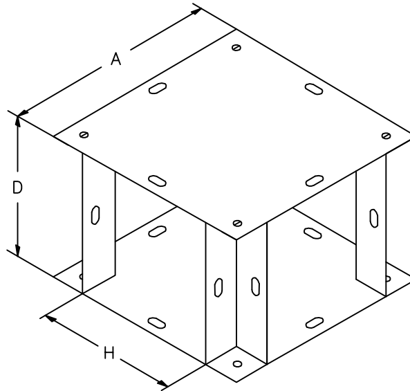
90 ELBOW-T-CROSS
