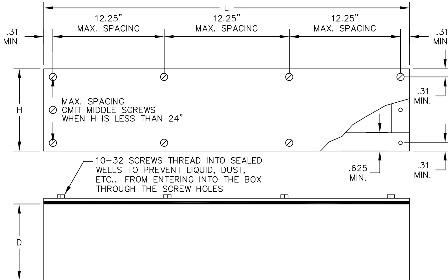
TYPE 3 AND TYPE 12 GASKETED WIRING TROUGH
