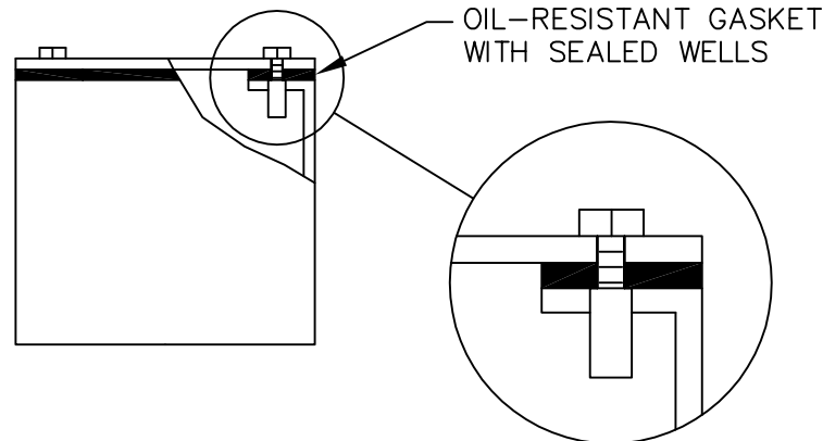
TYPE 3 AND TYPE 12 GASKETED WIRING TROUGH
